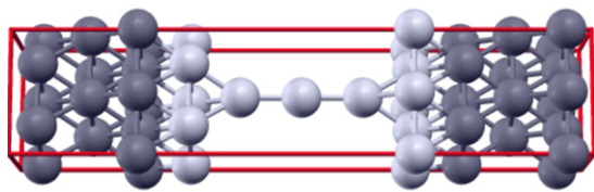
Figure 16. Three atom gold chain: supercell geometry showing the atomic wire connected to two gold electrodes (Au 111 surfaces). The dark atoms indicate the region where dissipative coupling is present. Periodic boundary conditions are applied in all directions. The lateral interaction between a wire and the nearest periodic images has negligible effect on the current.
